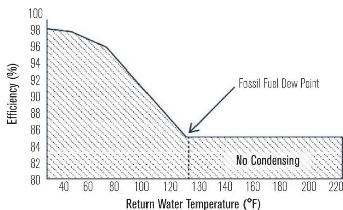
Figure 9: Flue gas condensation temperature and boiler efficiency
