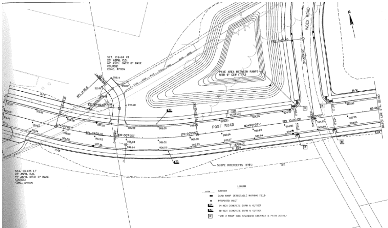
Copy of the proposed plans, Sheet C-221
